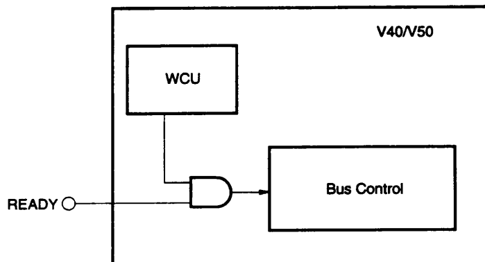
Figure 7-2. WCU and READY Control
