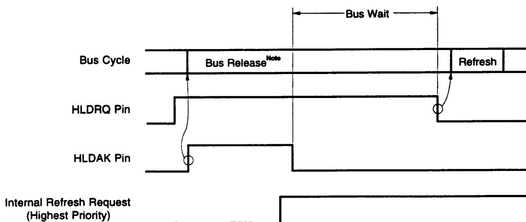
Figure 6-2. Bus Wait Operation
