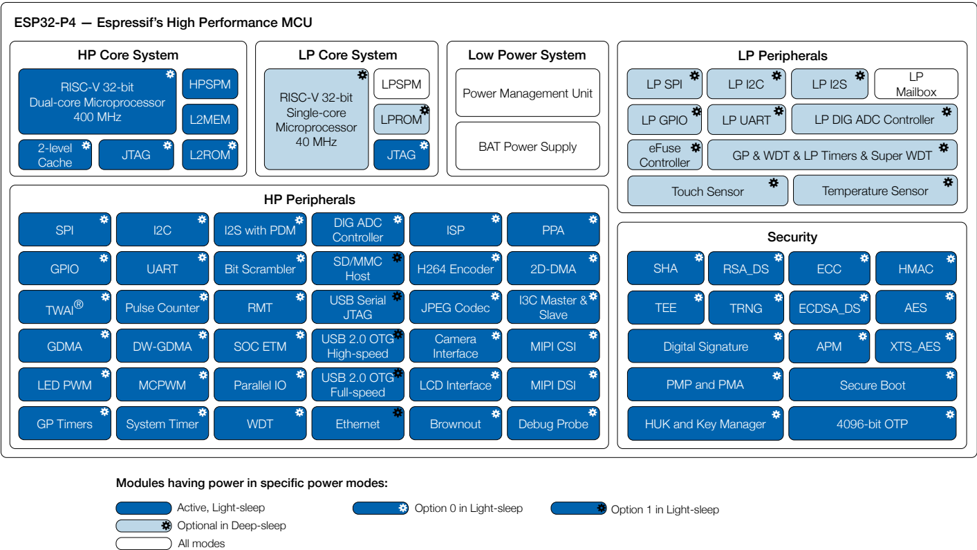
ESP32-P4 Functional Block Diagram
